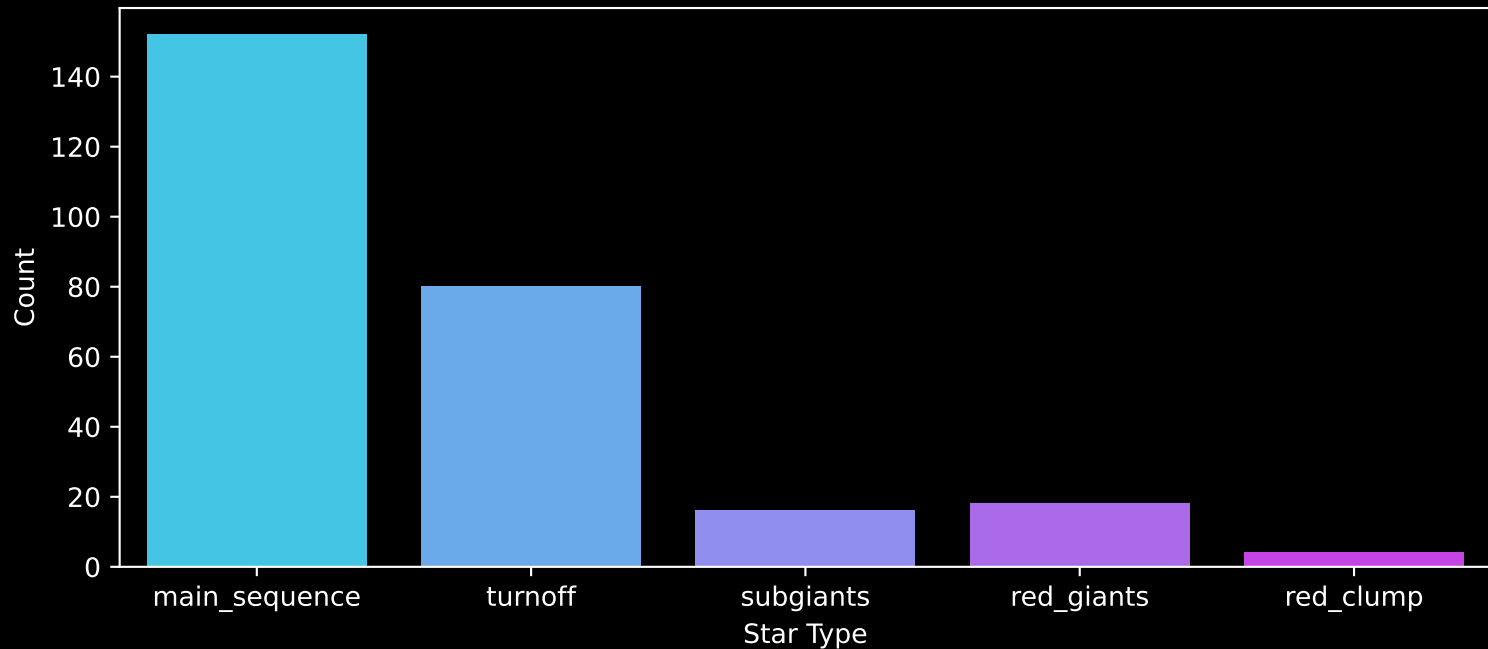
GALAH DR4 Field: [669] Count plot of Star Type
