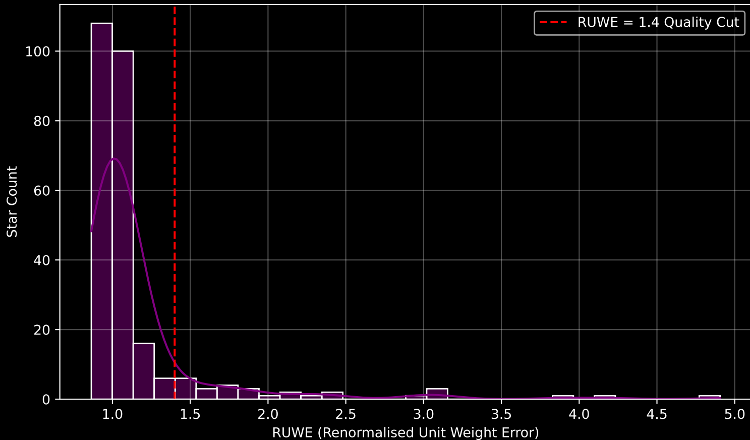
GALAH DR4 Field [669] RUWE Distribution (n= 259)
